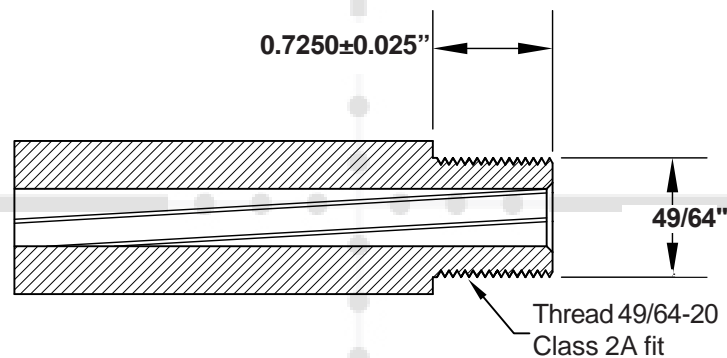
Barrel Threading Specifications
